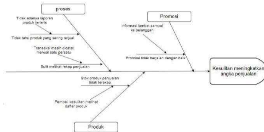
Gambar 3.1 Fishbone Diagram
