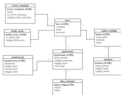
Gambar 11. Class Diagram
