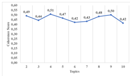
Fig. 3. Comparison of coherence score.
