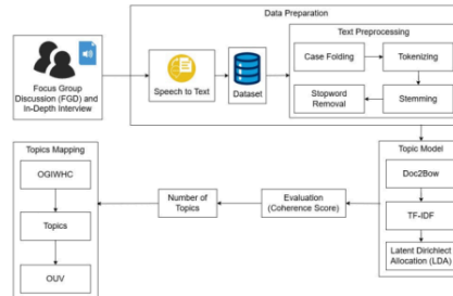
Fig. 1. Proposed methodology.
