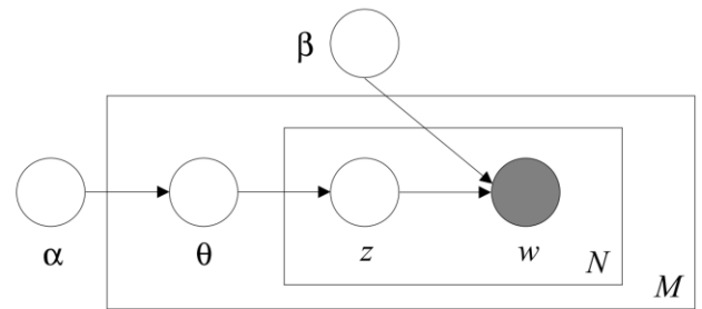
Fig. 2. LDA Model Diagram [23]
