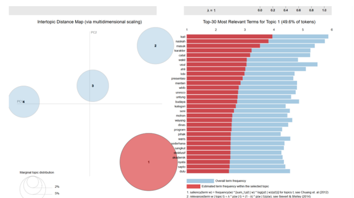
Fig. 5. Model visualization of topic 1.
