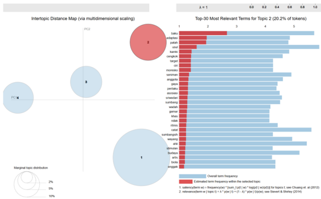
Fig. 7. Model Visualization of Topic 2
