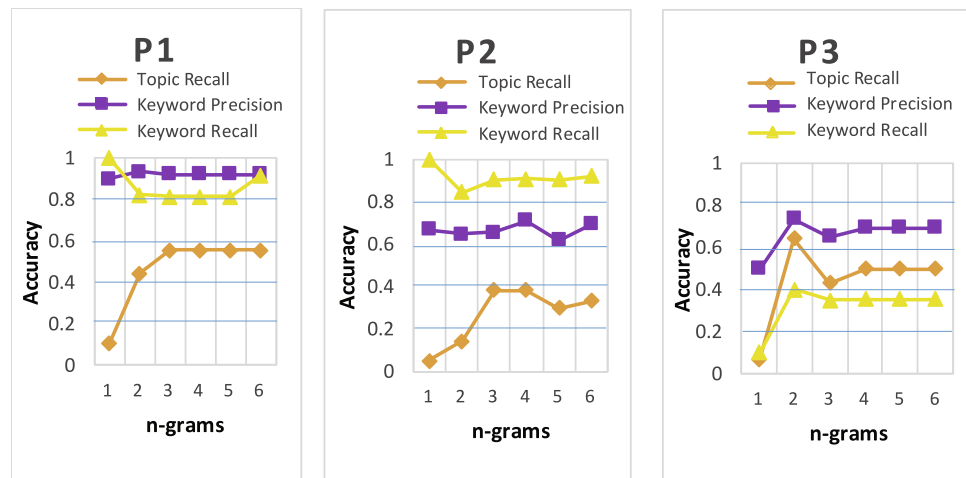
Fig. 4. The effect of n -grams variation on accuracy.
