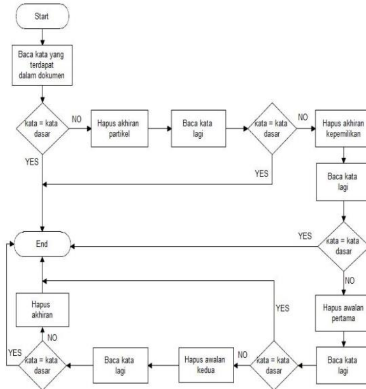
Gambar 3. Alur Proses Stemming
