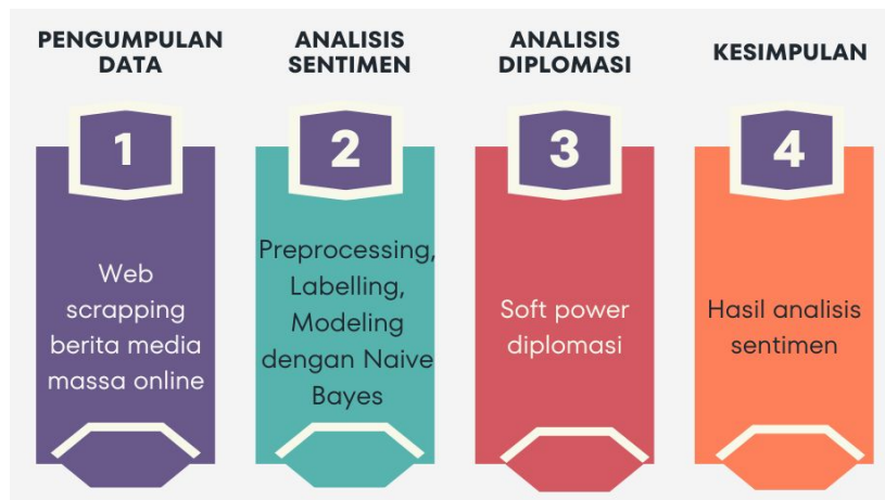
Gambar 1. Alur Penelitian
