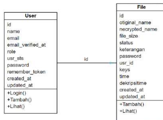
Gambar 2. Class Diagram
