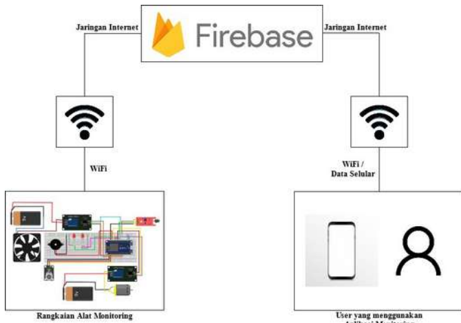
Gambar 3. Deployment Diagram
