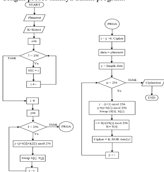
Gambar 5. Flowchart Enkripsi RC4
