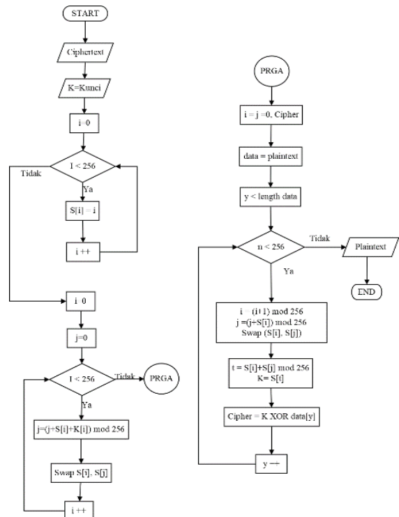
Gambar 6. Flowchart Dekripsi RC4
