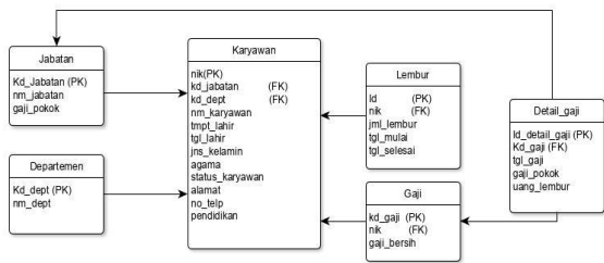
Gambar 3. LRS (Logical Record Structured)
