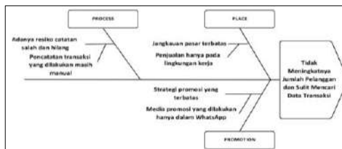
Gambar 2. Fishbone Diagram
