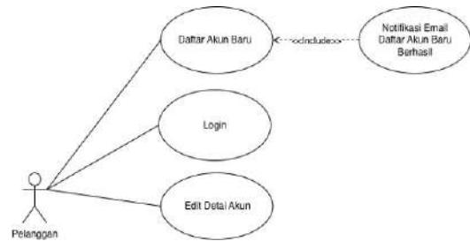
Gambar 5. Diagram Use Case Master Pelanggan
