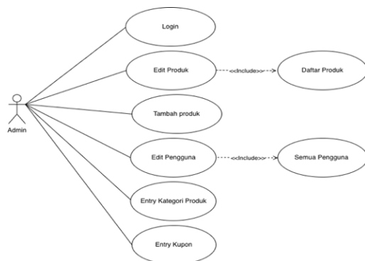
Gambar 4. Diagram Use Case Master Admin
