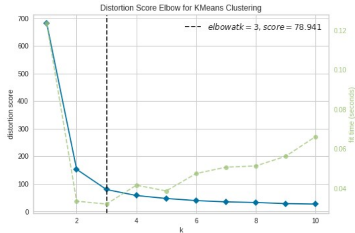
Gambar 3. Grafik Penentuan K-Cluster ( Elbow Method ) Dataset Honeypot
