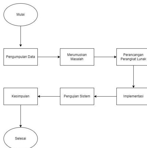
Gambar 1 Metode Waterfall
