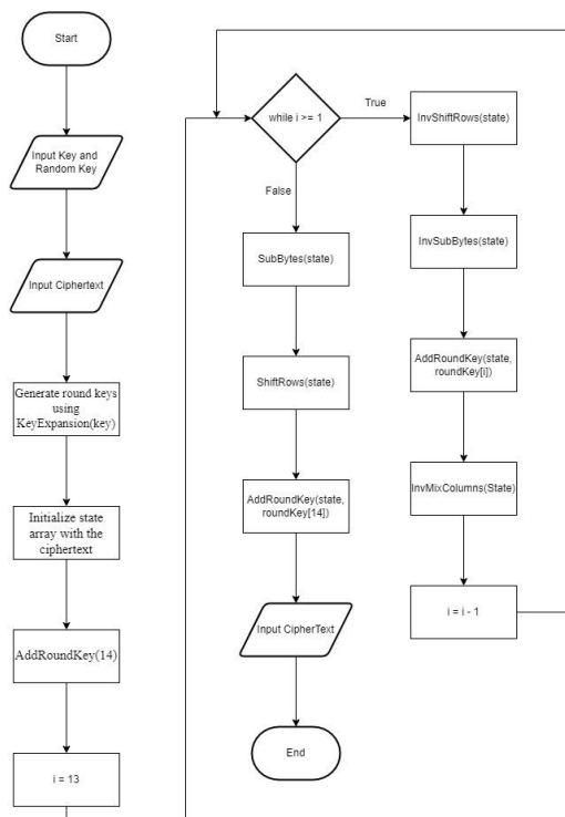
Gambar 5 Flowchart Tahapan Dekripsi
