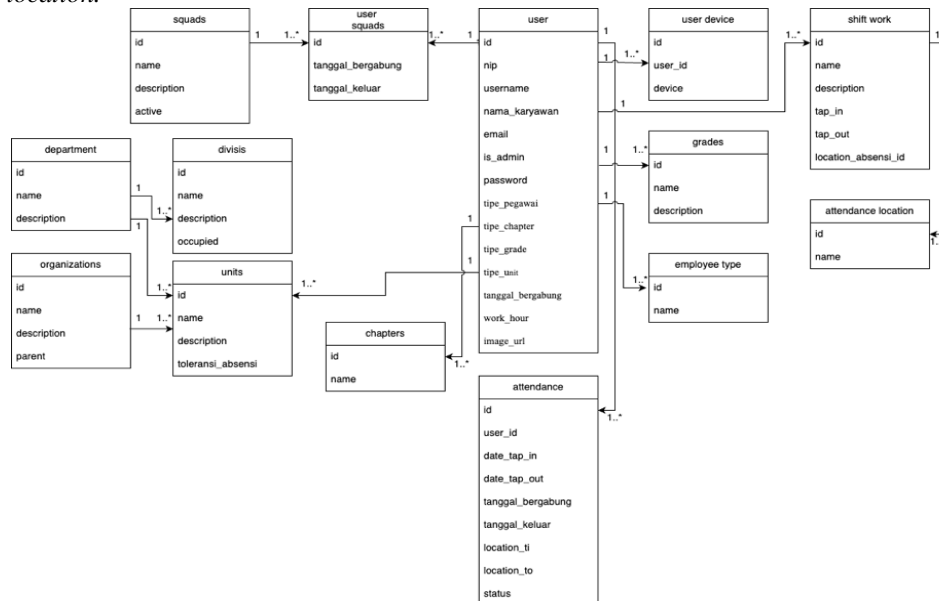
Gambar 5. Class Diagram
