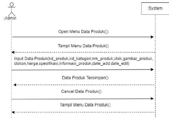
Gambar 10. Sequence Diagram Data Produk
