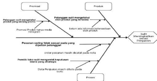
Gambar 3. Fishbone Diagram
