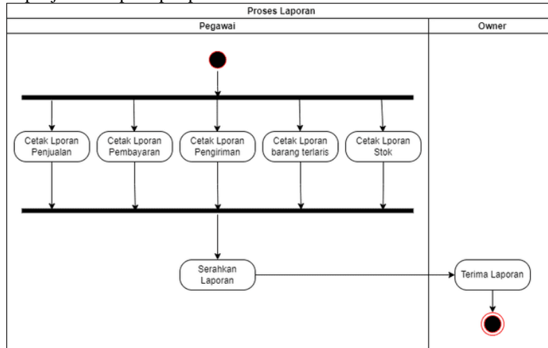
Gambar 7. Activity Diagram Sistem Usulan Proses Laporan
