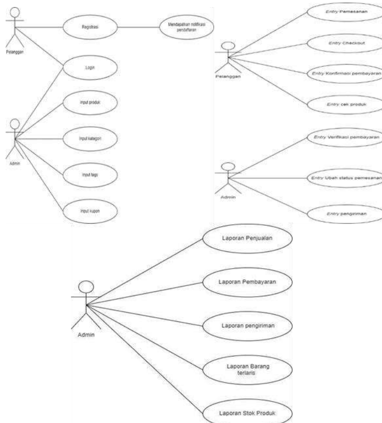
Gambar 8. Use Case Diagram
