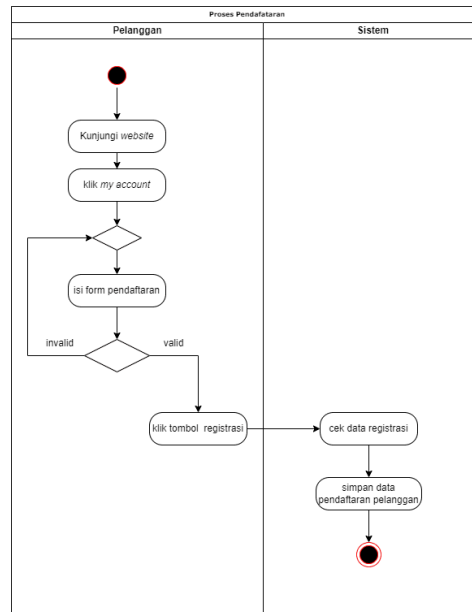
Gambar 3. Activity Diagram Sistem Usulan Proses Pendaftaran
