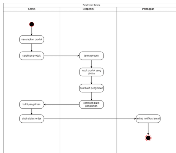
Gambar 6. Activity Diagram Sistem Usulan Proses Pengiriman
