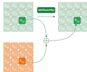
Gambar 1. AddRoundKey
