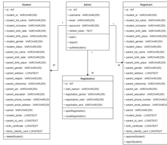
Gambar 5. Class Diagram
