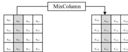
Gambar 4. MixColumn
