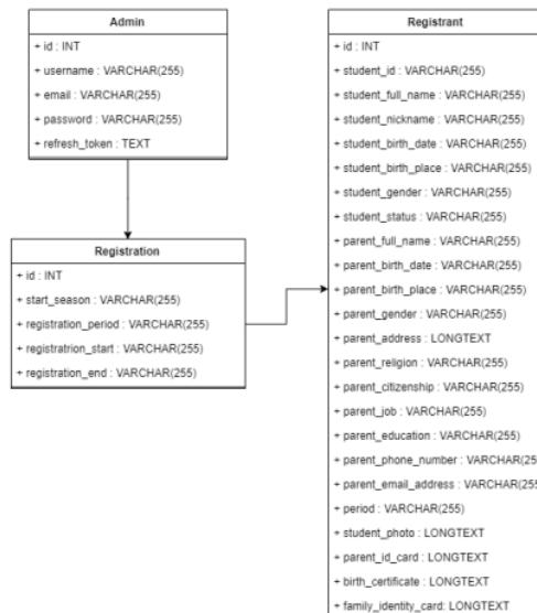
Gambar 6. Logical Record Structure (LRS)
