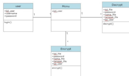
Gambar 4. Class Diagram User
