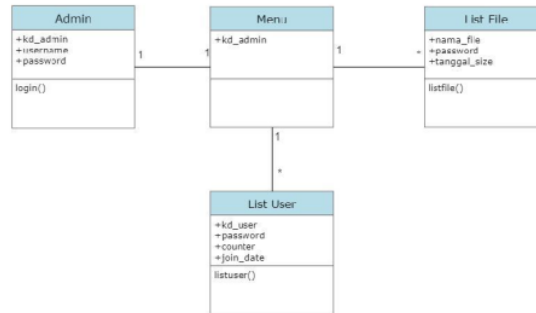
Gambar 3. Class Diagram Admin
