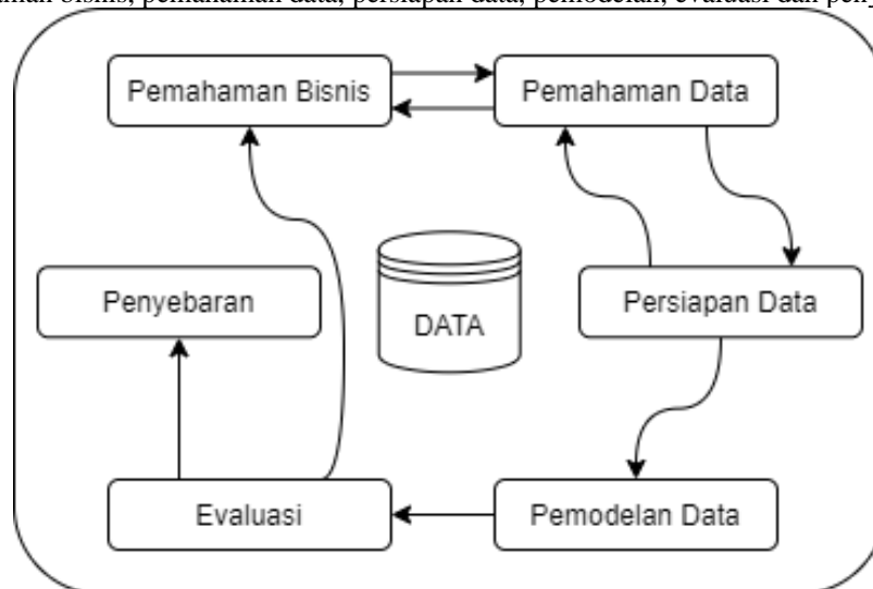
Gambar 1. Proses CRISP-DM[8]
