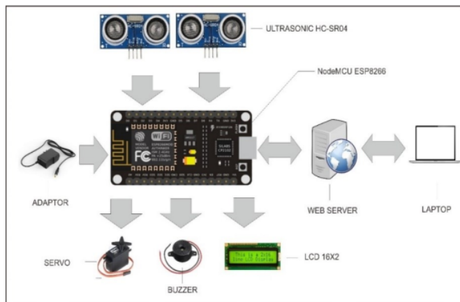
Gambar 3. Blok Diagram
