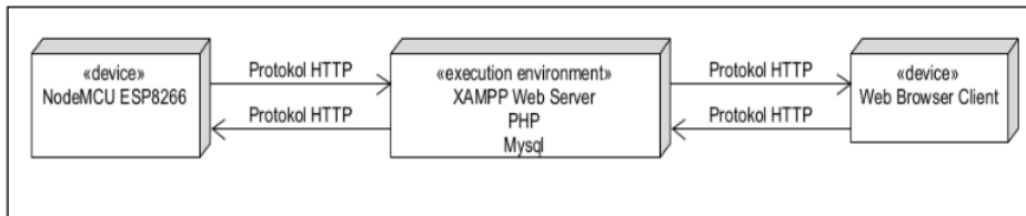
Gambar 5. Deployment Diagram
