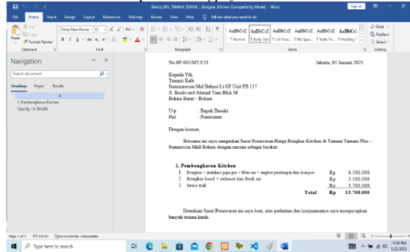
Gambar 8. Hasil Decrypt
