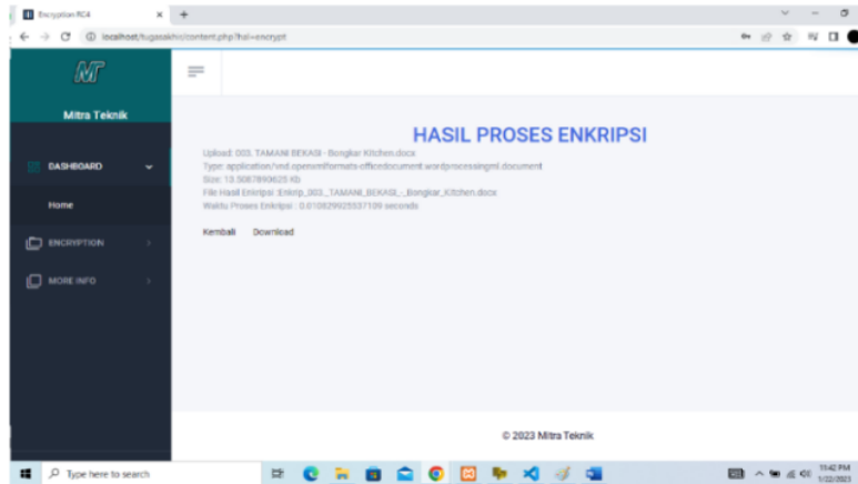
Gambar 5. Implementasi Encrypt
