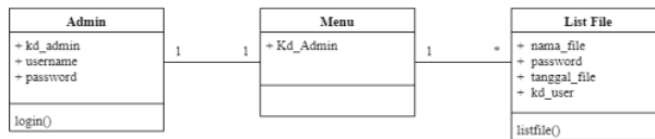
Gambar 2. Class Diagram Admin.
