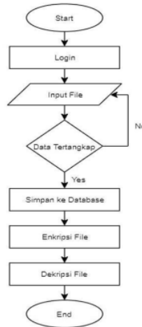
Gambar 1. Flowchart Sistem
