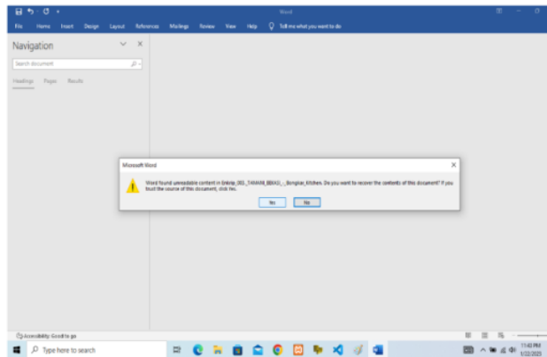
Gambar 6. Hasil Encrypt
