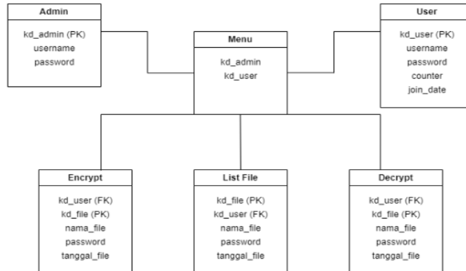
Gambar 4. LRS
