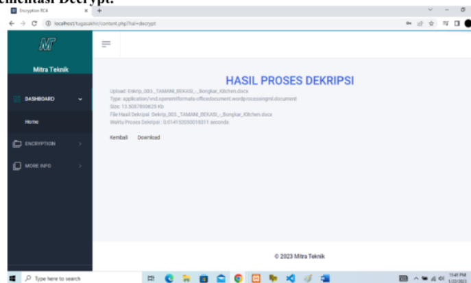
Gambar 7. Implementasi Decrypt
