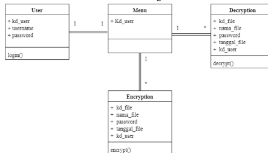
Gambar 3. Class Diagram User
