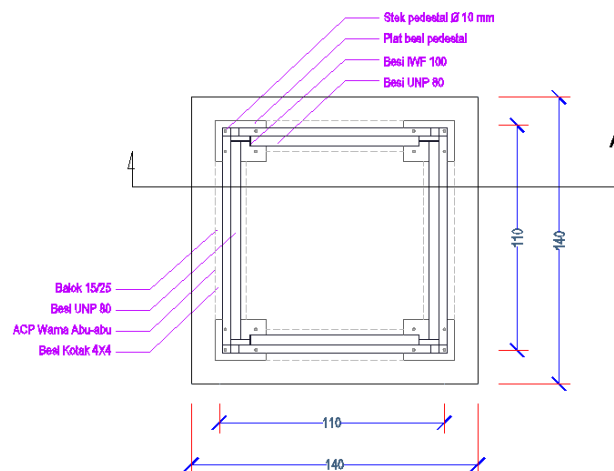
Gambar 11. Denah Minaret ( as built drawing ).
