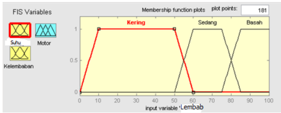
Gambar 3.8 Fuzzy Set Kelembaban Modul 2
