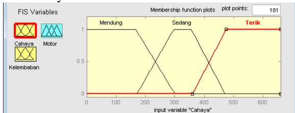
Gambar 3.3 Fuzzy Set Cahaya
