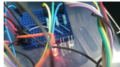
Gambar 4.9 Rangkaian LED Modul 1
