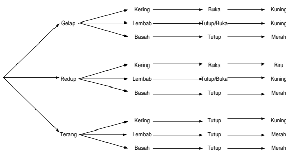
Gambar 3.10 Rule Fuzzy Cahaya-Kelembaban
