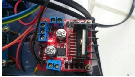
Gambar 4.5 Motor Driver
