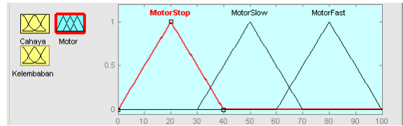
Gambar 3.5 Fuzzy Set Output Modul 1
