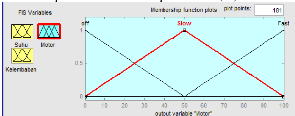
Gambar 3.9 Fuzzy Set Output Modul 2
