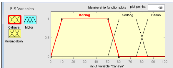
Gambar 3.4 Fuzzy Set Kelembaban Modul 1
