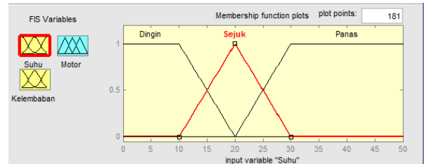
Gambar 3.7 Fuzzy Set Suhu
