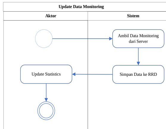
Gambar 6. Activity Diagram Update Data Monitoring
