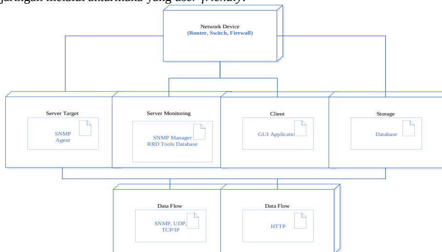
Gambar 9. Deployment Diagram Sistem
