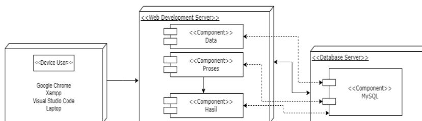
Gambar 2. Deployment Diagram
