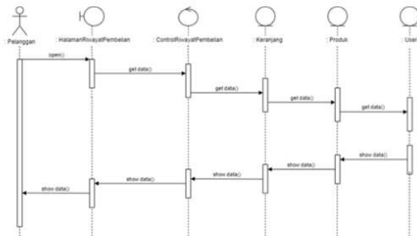
Gambar 19 Sequence Diagram Riwayat Pembelian
