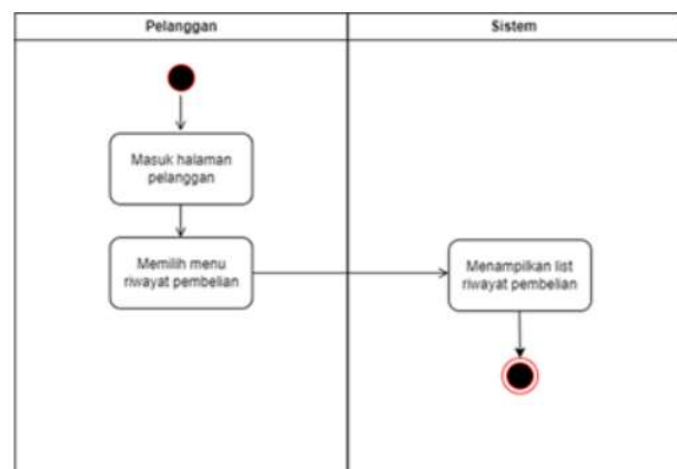
Gambar 9. Activity Diagram Riwayat Pembelian
