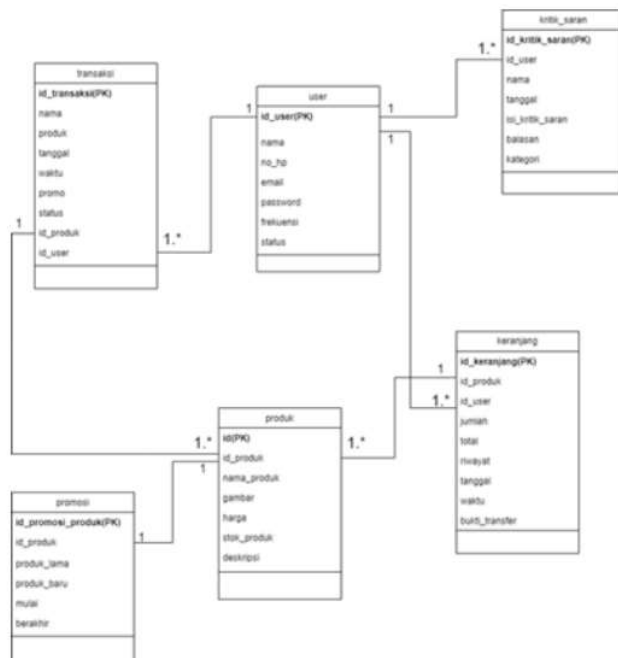
Gambar 11. Class Diagram
