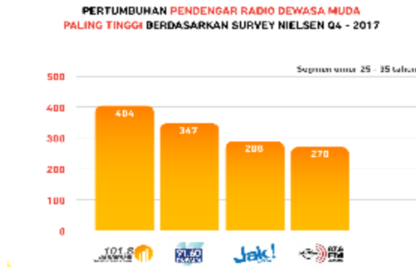
Gambar 1. Growth Listener
