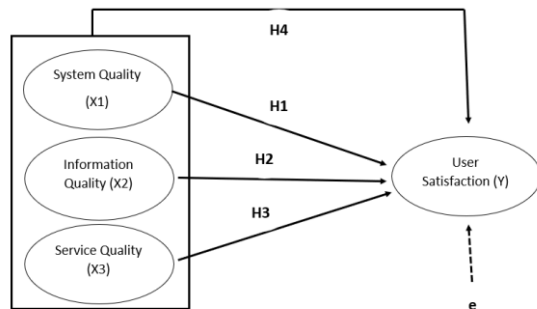
Figure 2. Research Framework
