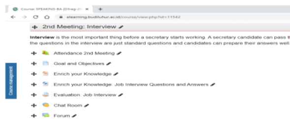
Image 1: Moodle Website
