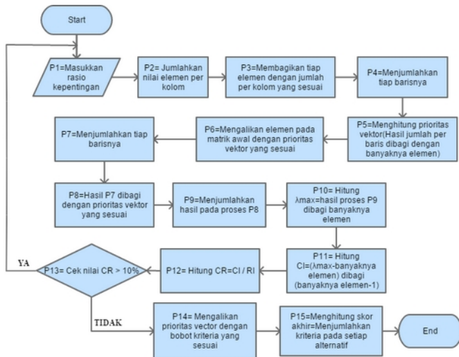
Gambar 5. Flowchart AHP
