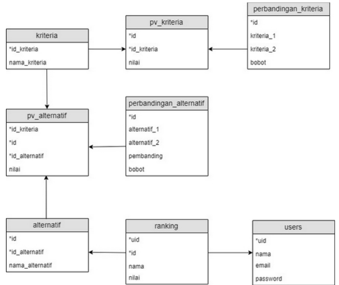
Gambar 4. Logical Record Structured
