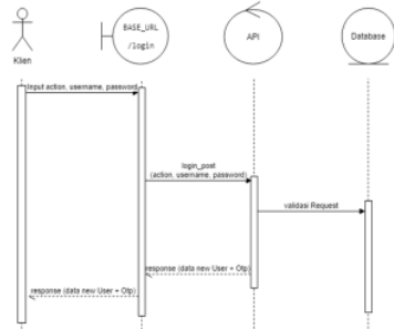
Gambar 3. Diagram Sequence Bagian Login
