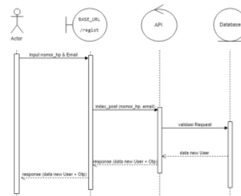
Gambar 2. Diagram Sequence bagian Registrasi
