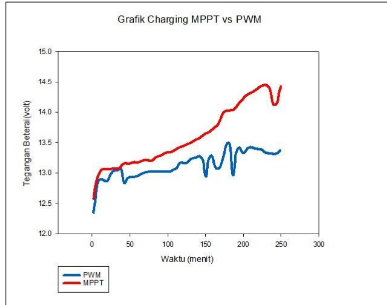
Gambar 5. Grafik Charging MPPT vs PWM
